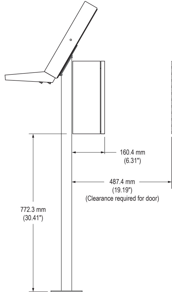
Side View
