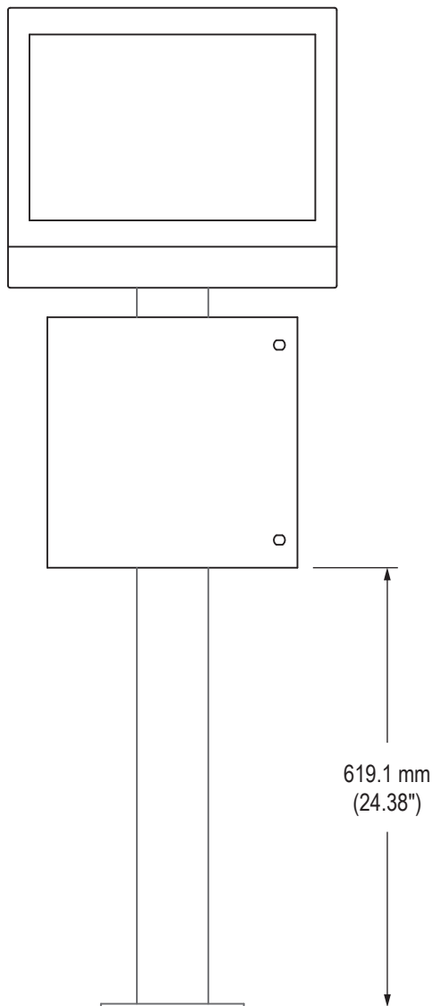
Front View
