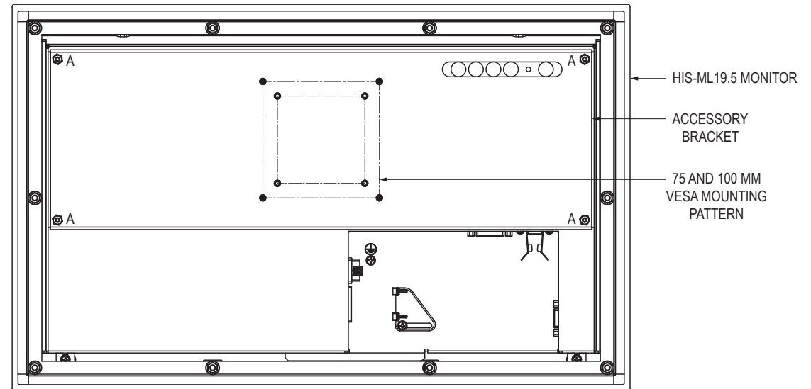
FIGURE 1 – REAR VIEW OF ML19.5 MONITOR (FACE DOWN)
