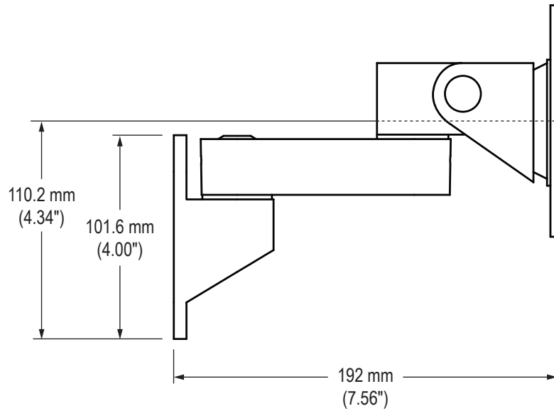
Side View with 3.5" Extension Arm
