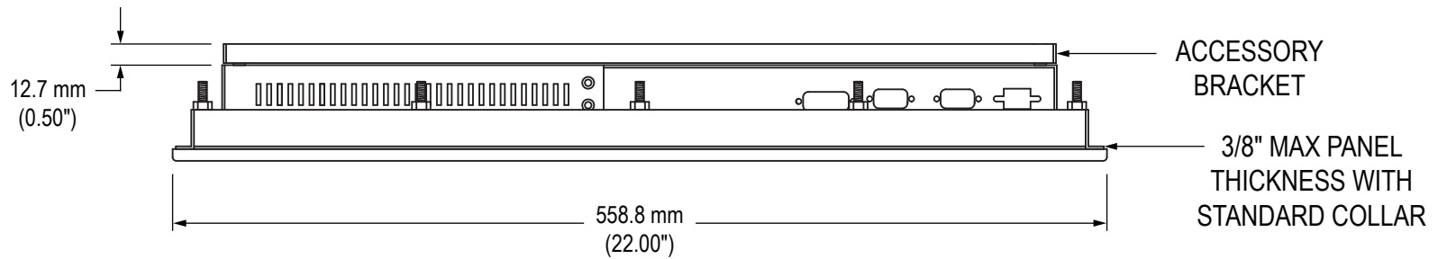
Bottom View
