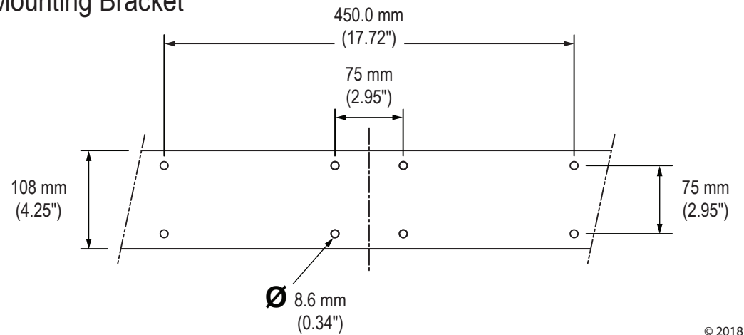
Mounting Bracket
