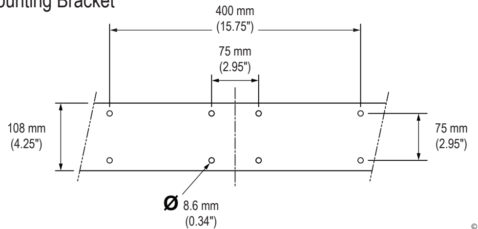
Mounting Bracket
