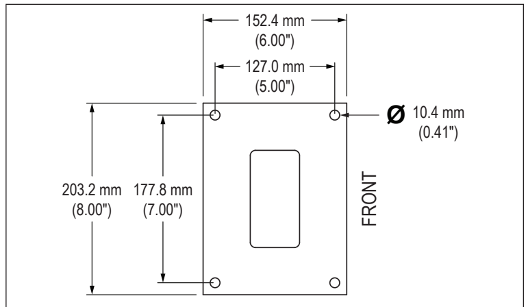
FIGURE 1 – PEDESTAL BASE PLATE
