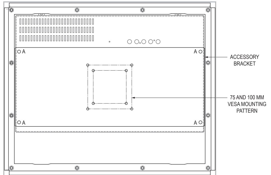
FIGURE 1 – REAR VIEW OF ML20 MONITOR (FACE DOWN)
