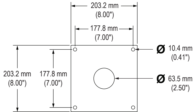
Pedestal Plate (in bottom of Pedestal for hidden cable access)
